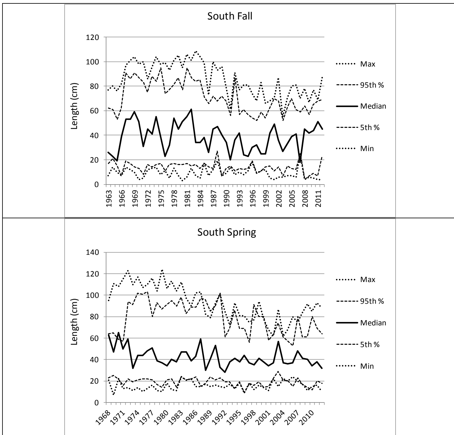
Figure 18. Length quantiles for monkfish over time from NEFSC autumn and spring surveys.
