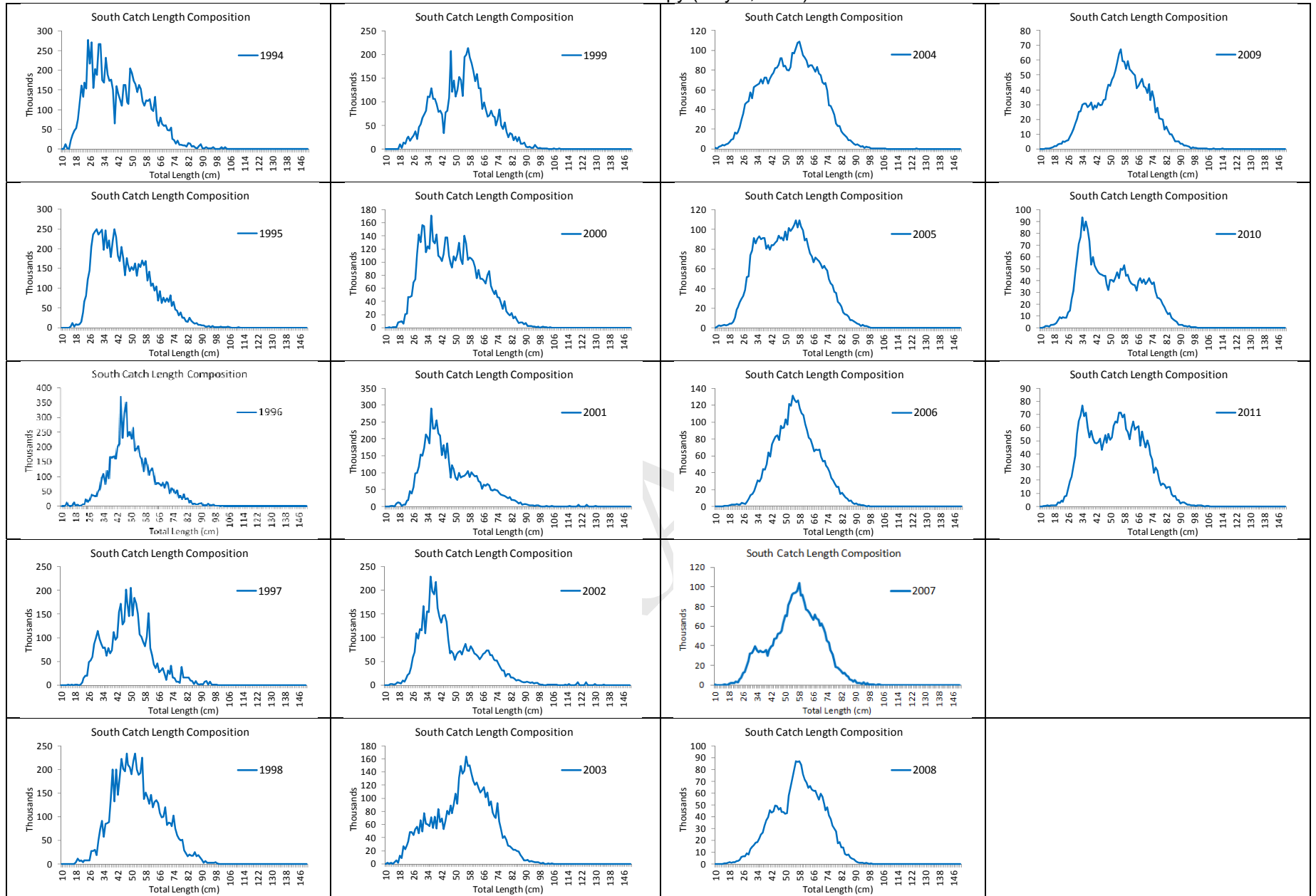
Figure 9. Length composition of monkfish commercial catch estimated using length frequency data collected by fishery observers in the southern management region.
