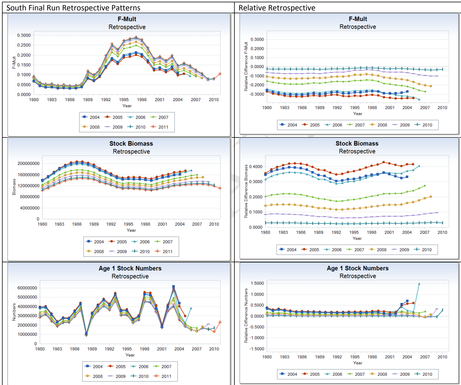
Figure 33. Retrospective patterns in the final SCALE model for the south, 7 peels.
