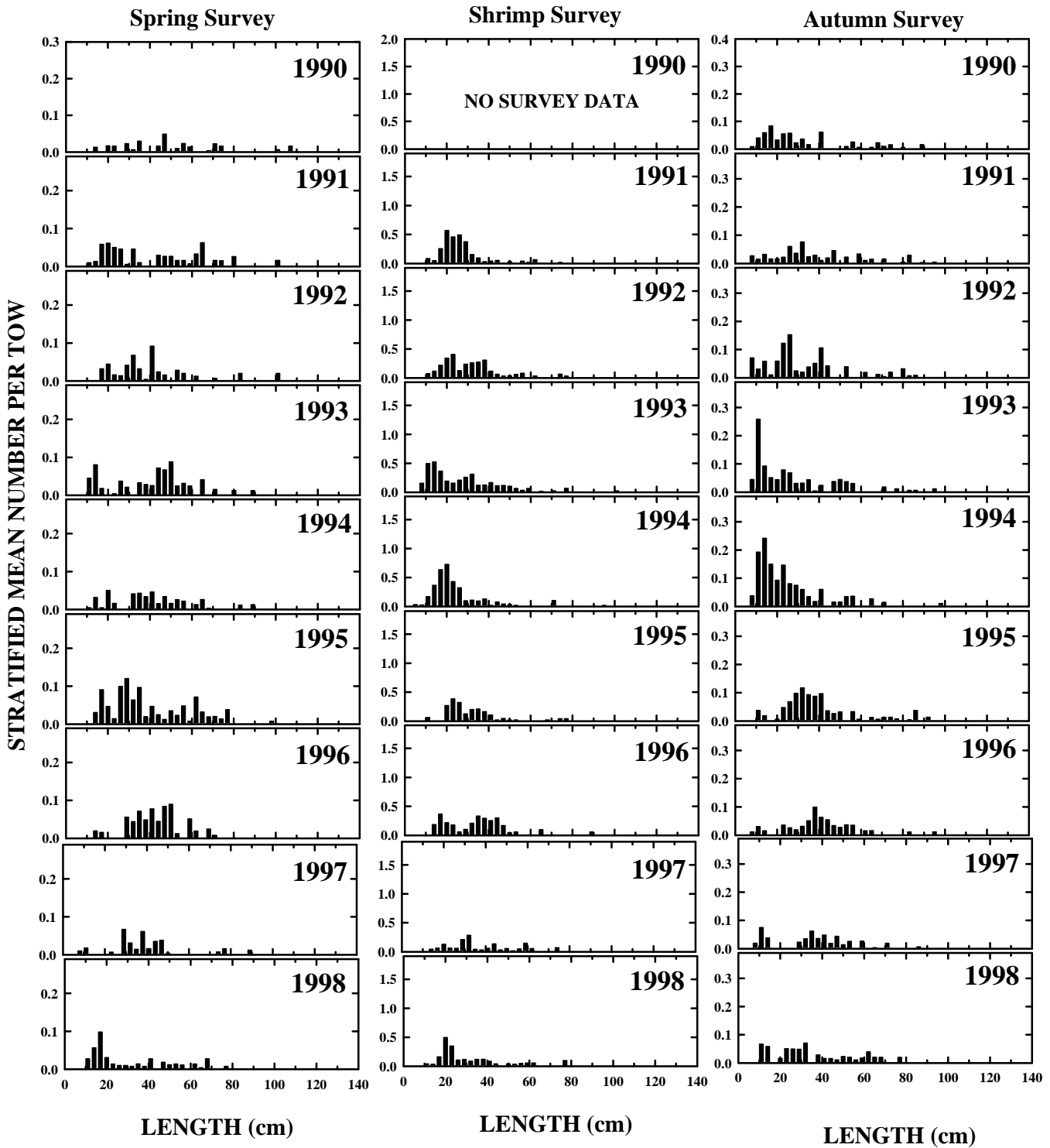
Figure 12d, continued. Goosefish length composition from the NEFSC spring and autumn bottom trawl survey, and ASMFC summer shrimp survey in the northern management region.
