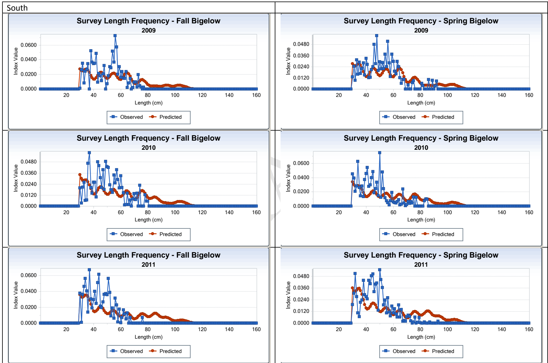
Figure 30. South SCALE final model fits to Bigelow survey length frequencies, 2009-2011
