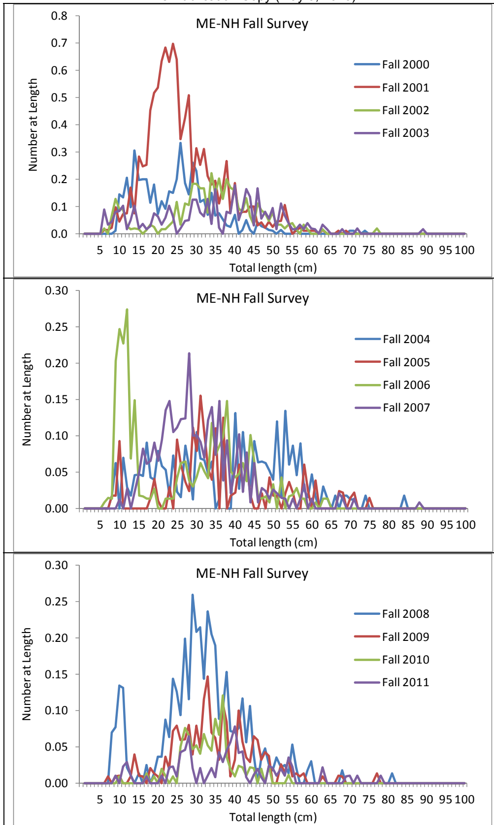
Figure 15. Length frequencies from Maine-New Hampshire fall inshore survey, 2000-2011.
