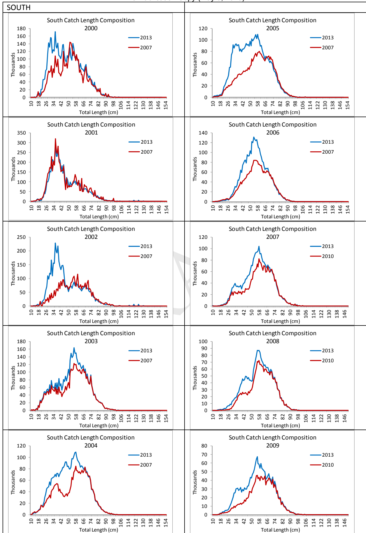
Figure 9. Revisions to catch length composition, South. sbrm_discard/2013_sbrm/2010 vs 2013.xls/est If cf S
