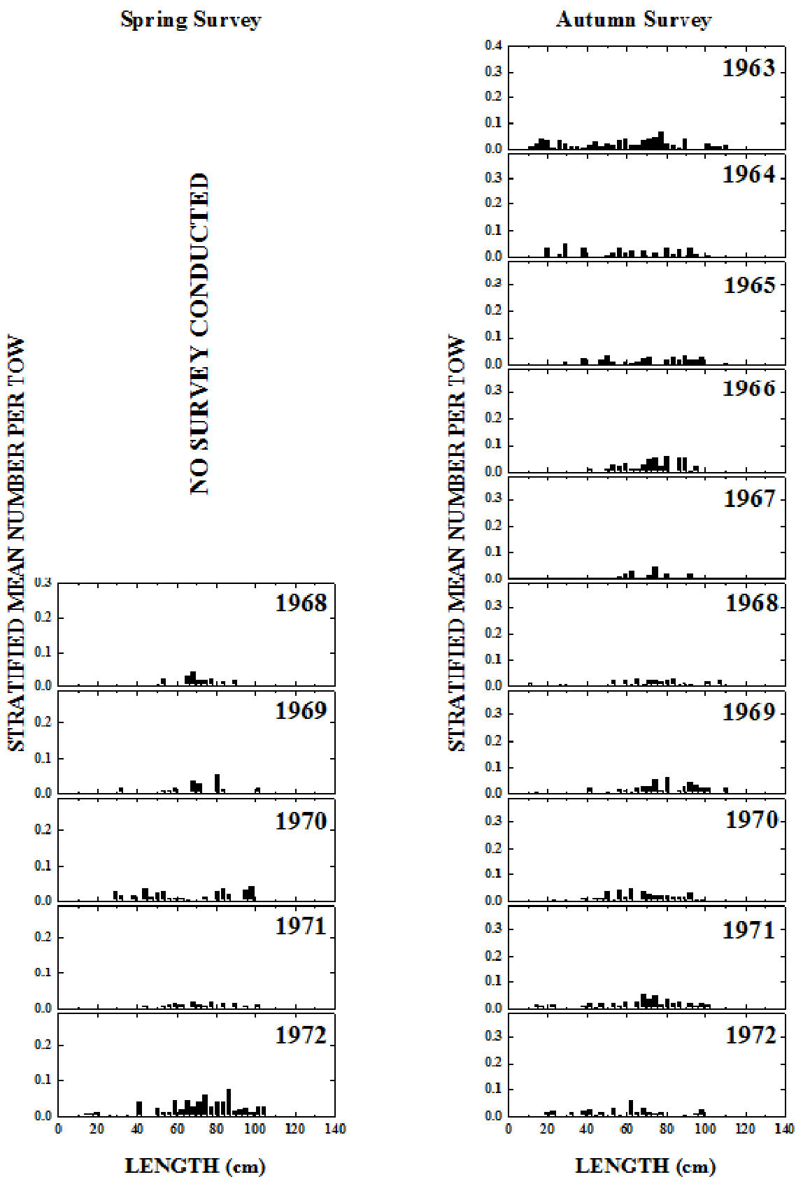
Figure 12a. Goosefish length composition from the NEFSC spring and autumn bottom trawl surveys in the northern management region.
