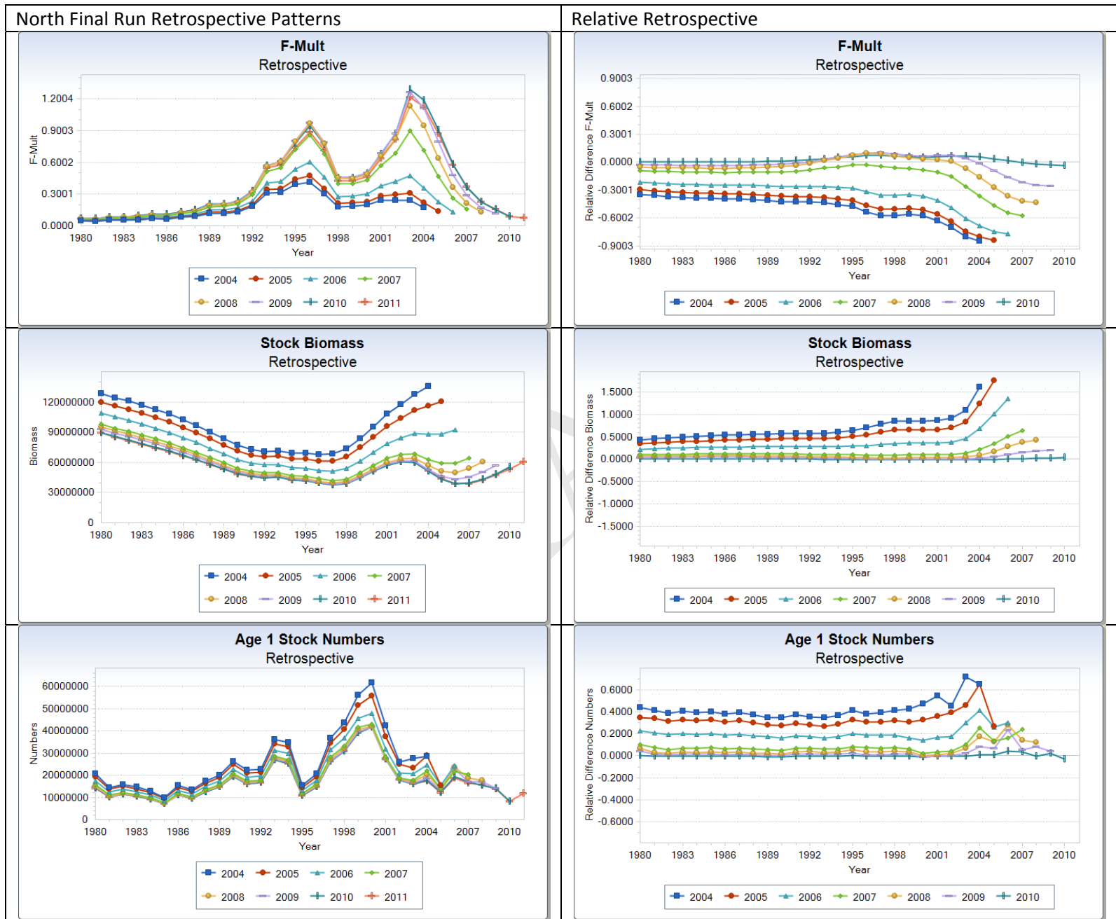
Figure 26. Retrospective patterns in final SCALE model for the north, 7 peels.
