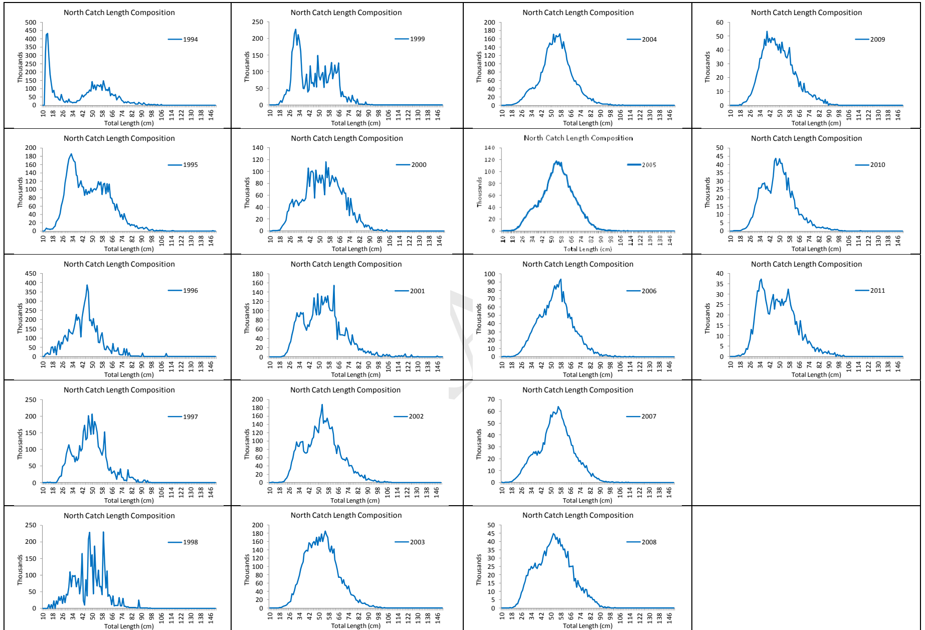
Figure 8. Length composition of monkfish commercial catch estimated using length frequency data collected by fishery observers in the northern management region.
