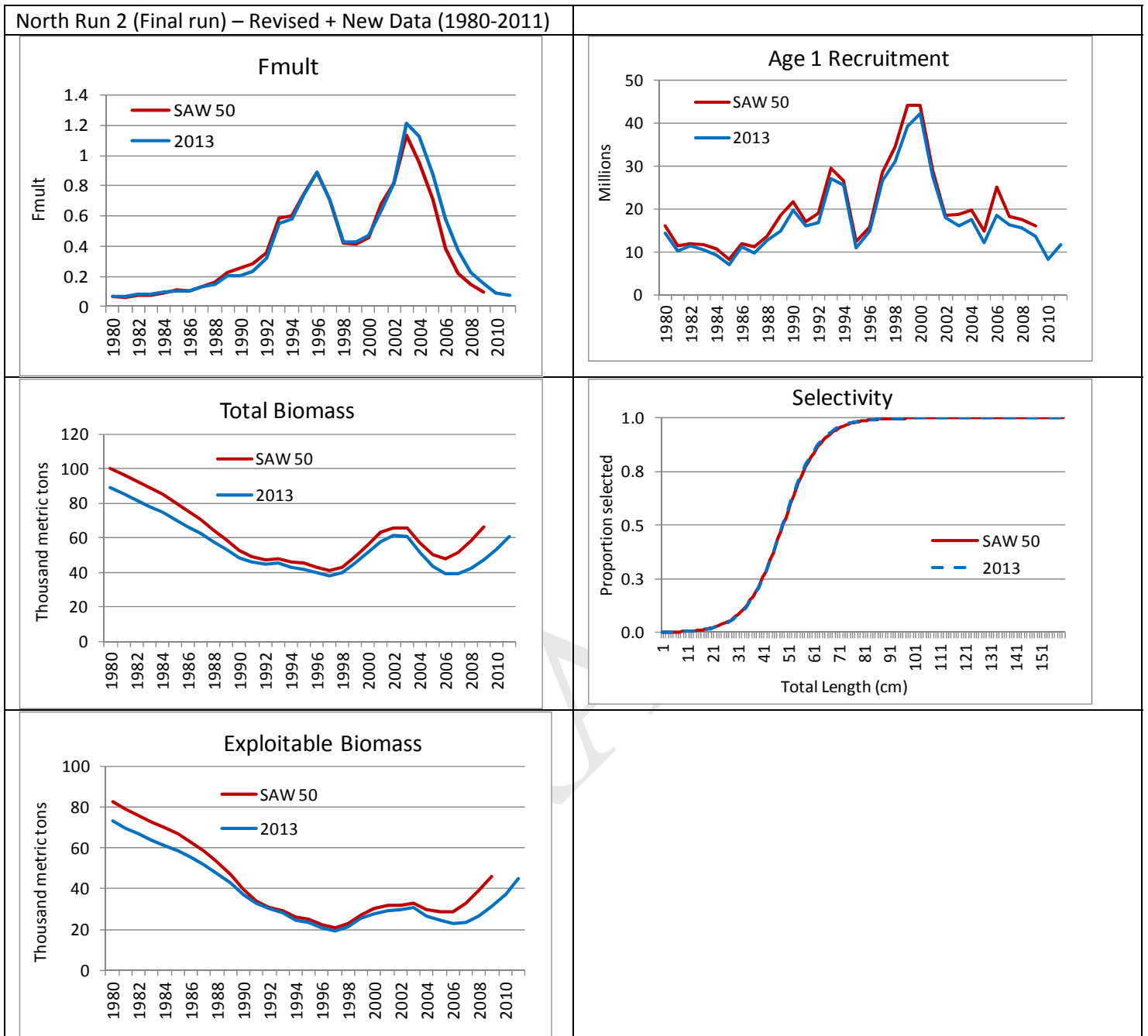
Figure 22. Comparison of SAW 50 SCALE model results for the North with results of same model using revised data (1980-2009) plus two additional years of data (2010-2011, final model for the North).
