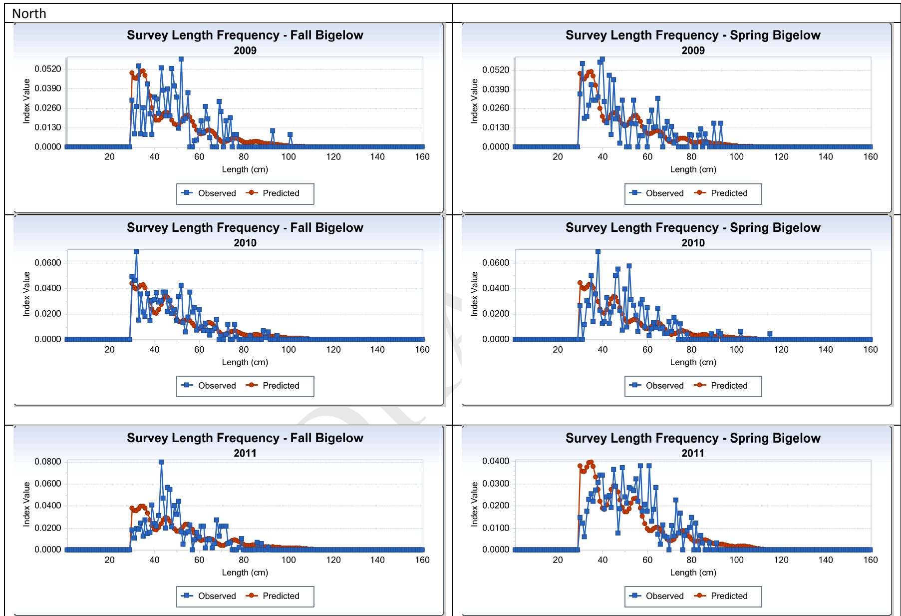
Figure 23. North SCALE final model fits to Bigelow survey length frequencies, 2009-2011.
