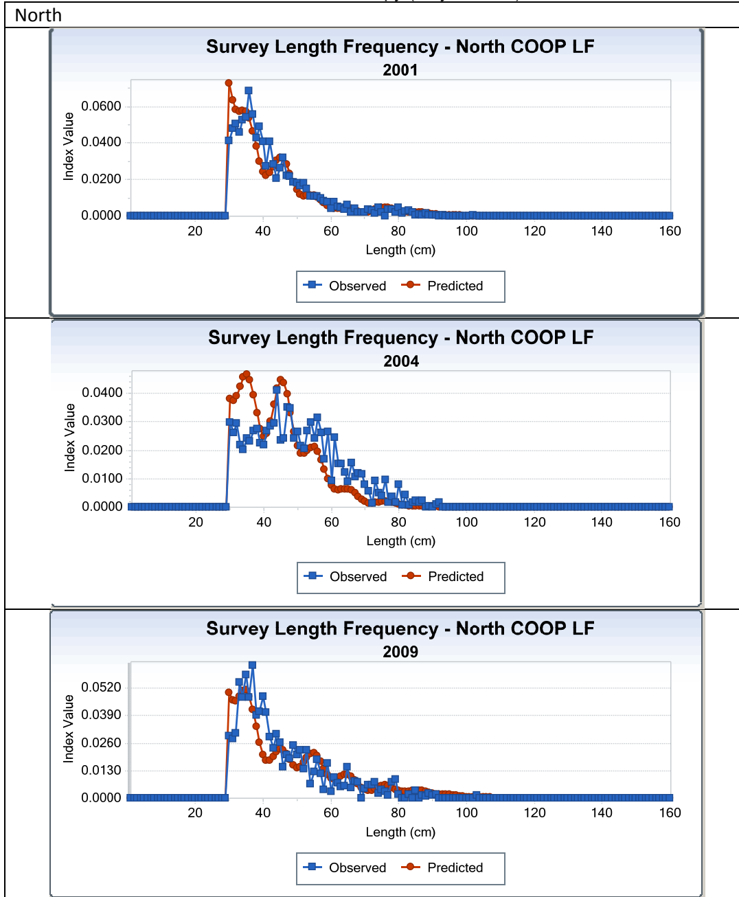
Figure 24. North SCALE model fits to Cooperative Monkfish Survey length frequencies, 2001, 2004, 2009.
