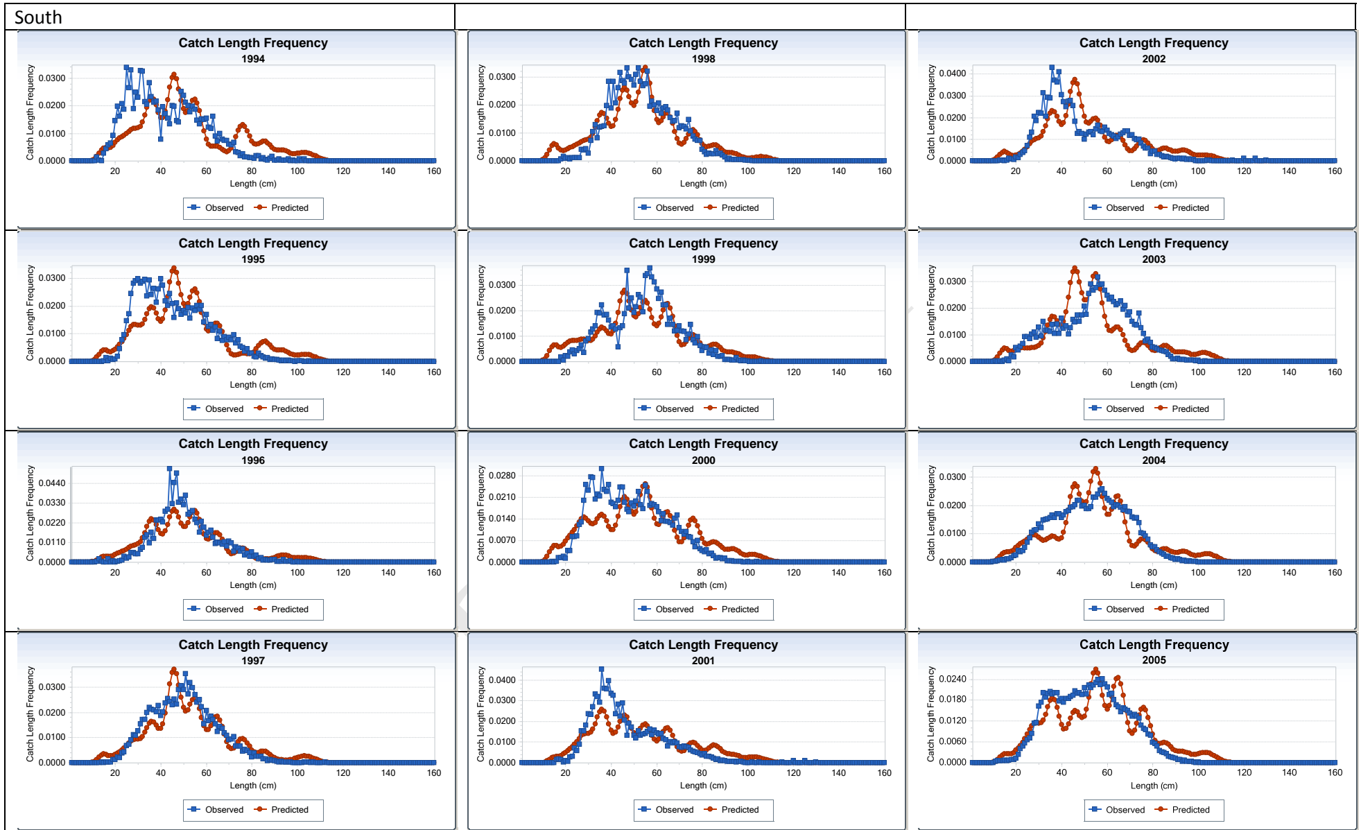
Figure 32a. South SCALE final model fits to catch length frequencies, 1994-2011.
