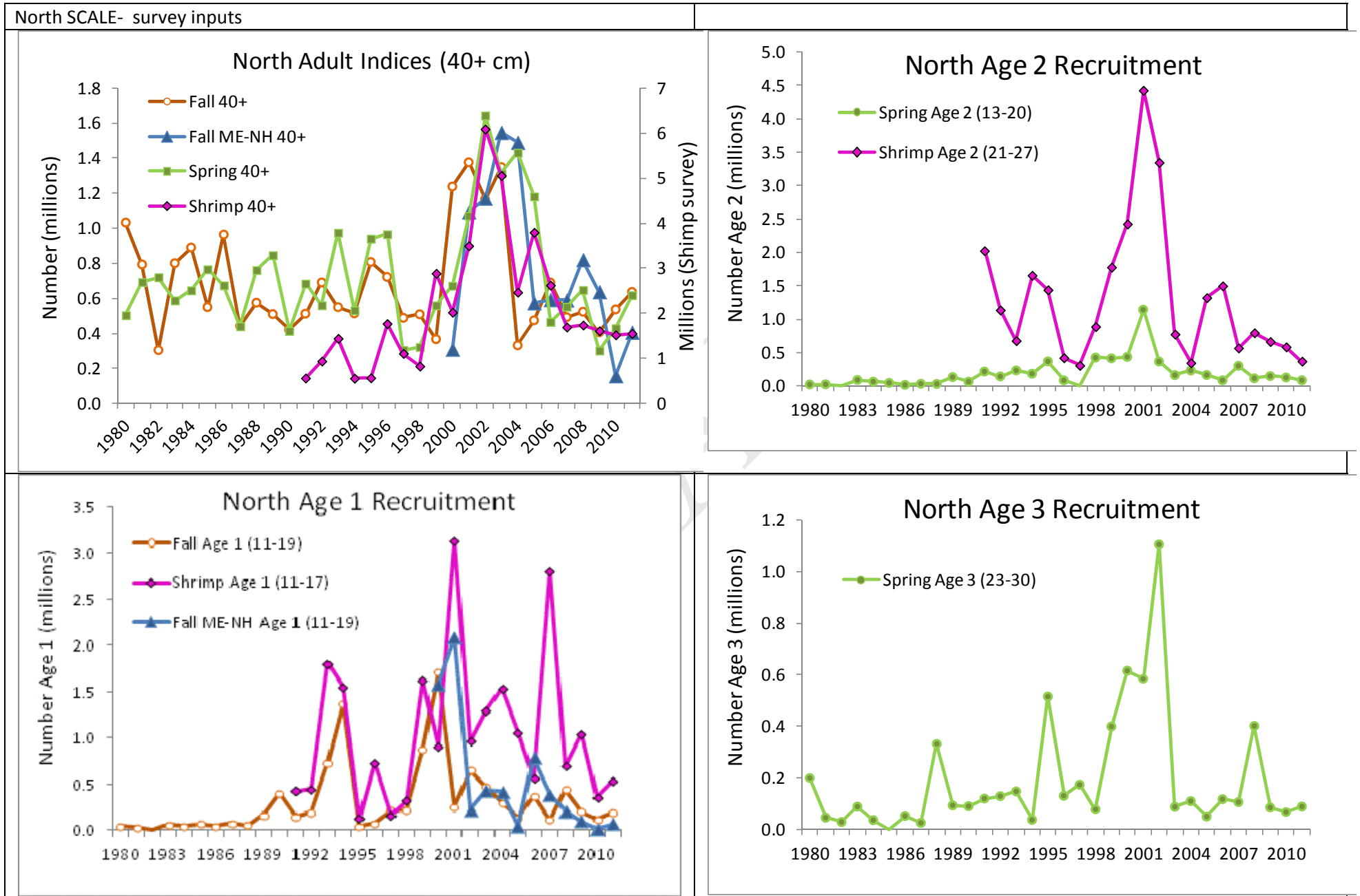
Figure 19. Survey inputs for the SCALe model for the northern management region.
