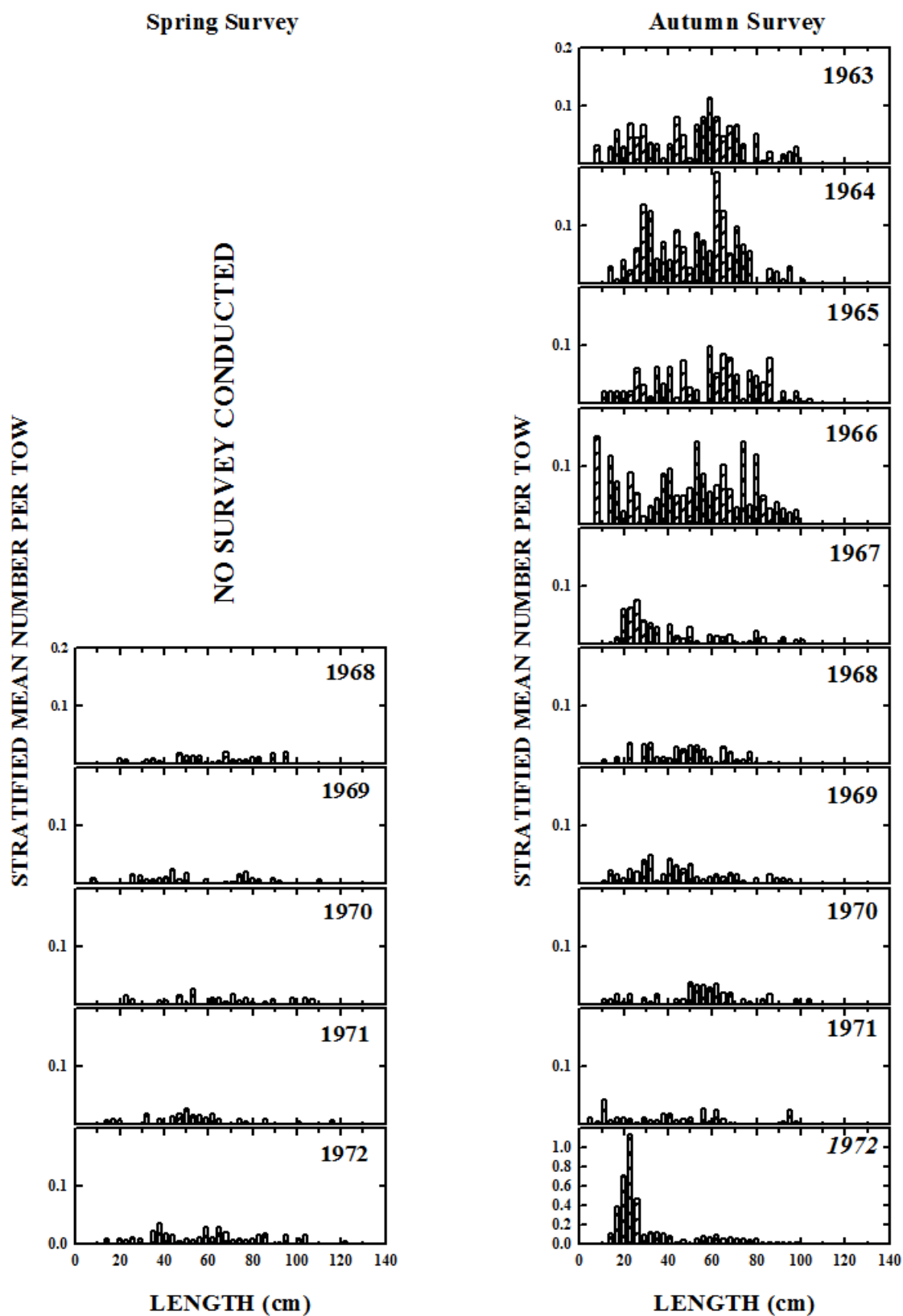
Figure 17a. Goosefish length composition from the NEFSC spring bottom trawl (March-April), winter flatfish (February), summer scallop (July-August), and autumn (September-October) bottom trawl surveys in the southern management region, 1963-2009. Note: 1963-1966 sampled reduced strata set.
