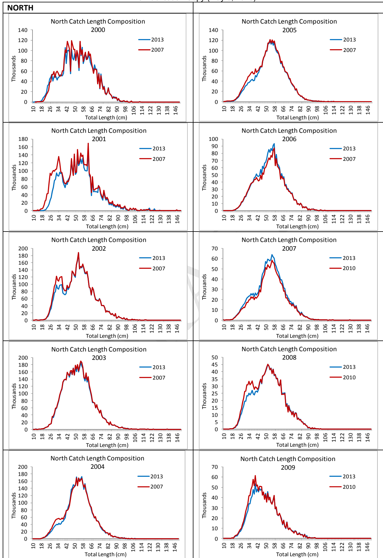
Figure 8. Revisions to catch length composition, North. sbrm_discard/2013_sbrm/2010 vs 2013.xls /est lf cf N
