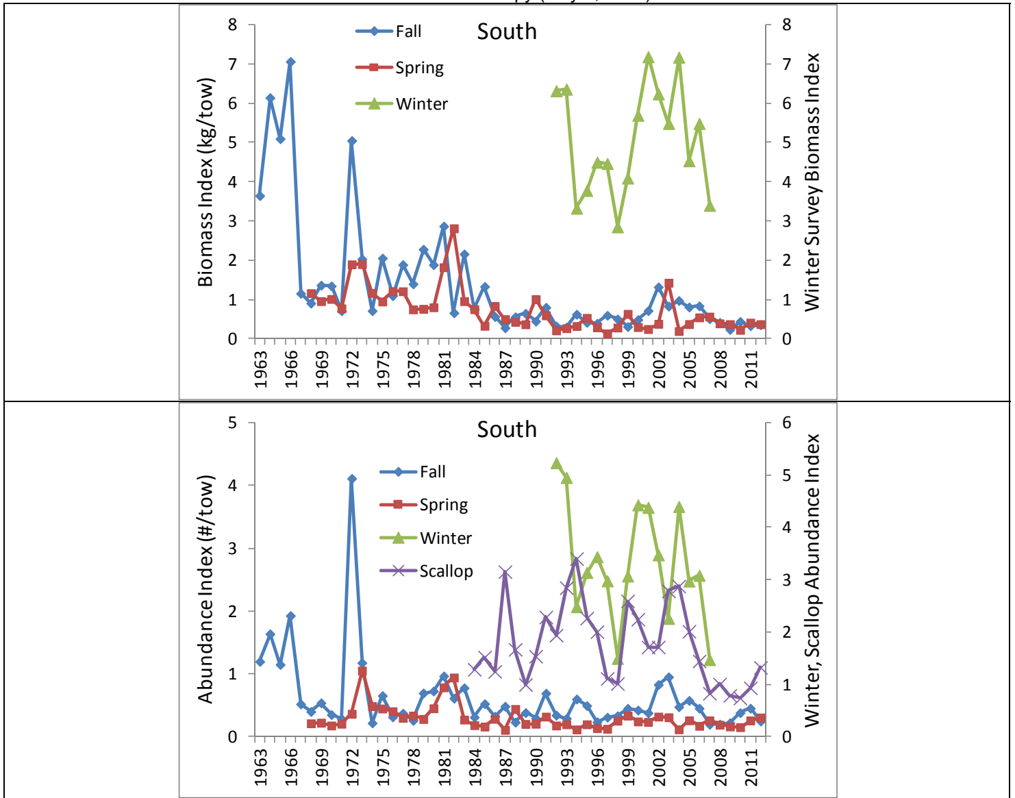
Figure 16. Survey indices for monkfish in the southern management area. Top panel biomass, bottom panel abundance.
