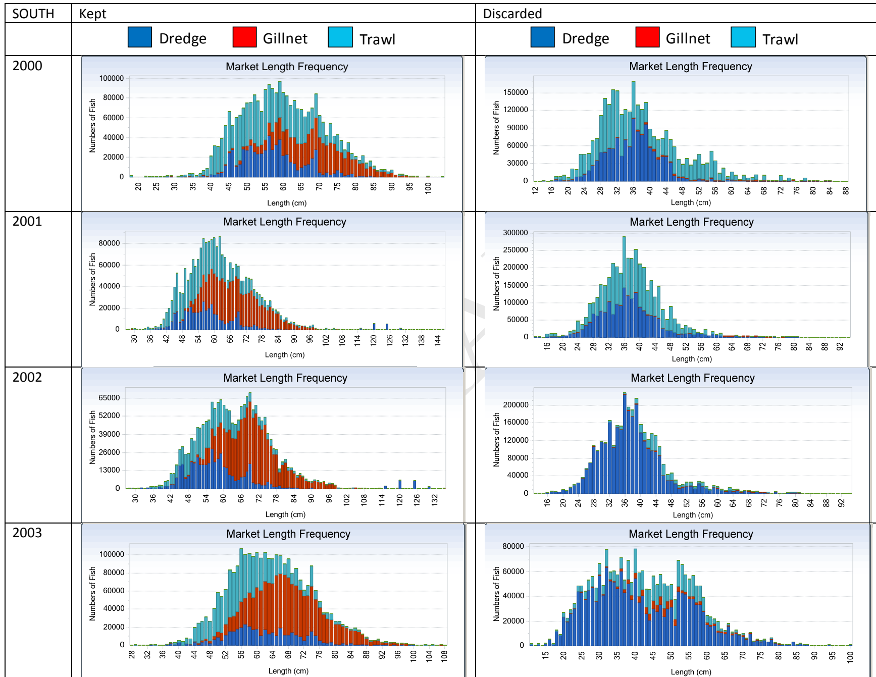
Figure 7a. Estimated length composition of kept and discarded monkfish in the South, by gear type.
